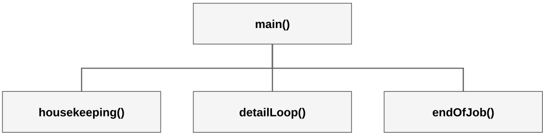
Hierarchy Chart
