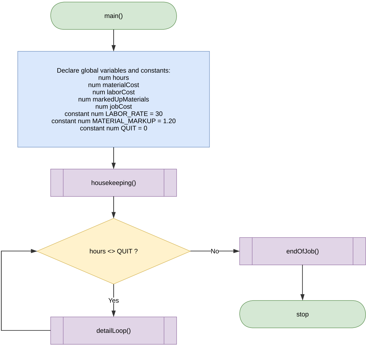
Main Program
